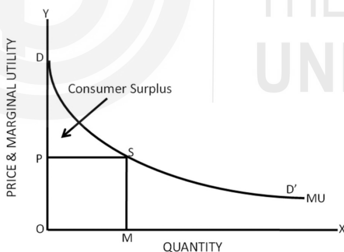
Fig. 4.6: Consumer Surplus
