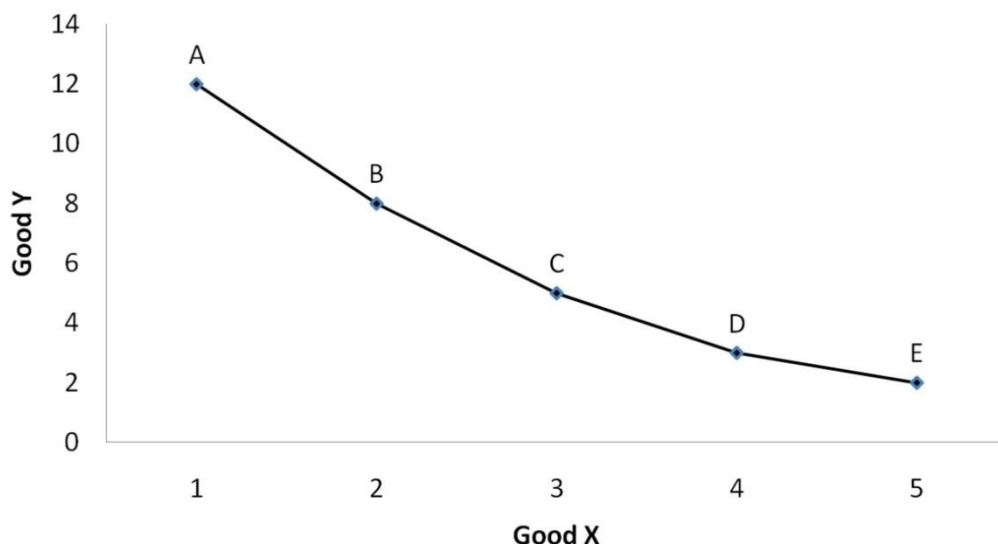
Fig. 5.1: Indifference curve
