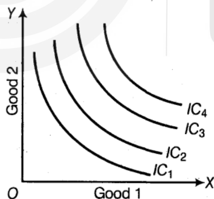
Fig. 5.2: Indifference map
